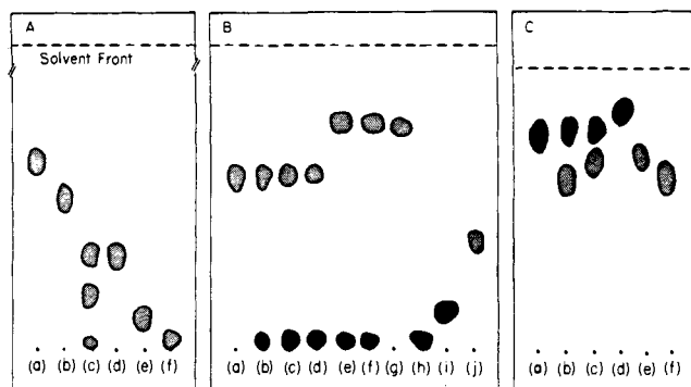
Figure 1. Tlc patterns of 1a metabolites and their degradation products. ○ = Fluorescence-quenching under 2537-Å lamp; ● = red after spraying with aniline phthalate reagent and heating at 110° for 0.5 hr. A. Silica gel HF 254 , CMA-II. (a) 1b; (b) 1c; (c) crude nucleoside fraction from rabbit urine after administration of 1a; (d) 1a; (e) 5; (f) 3'-amino-3'-deoxyinosine. The patterns were essentially reversed on Silicar tlc 7-GF with 88% HCO 2 H-abs EtOH-H 2 O (3:16:3). B. Silicar tlc 7-GF, CMA-I. (a) 6-Methylaminopurine; (b) major nucleoside metabolite (hydrolyzed = hyd); (c) acetylated metabolite (hyd); (d) synth 8 (hyd), (e) 1a (hyd); (f) acetylated 1a (hyd); (g) 6-dimethylaminopurine; (h) synth 3-amino-3-deoxy-D-ribose; (i) D-ribose; (j) adenine. C. Silicar tlc 7-GF, 88% HCO 2 H-abs EtOH-H 2 O (3:32:6). (a) Synth 3-amino-3-deoxy-D-ribose; (b) 1a (hyd); (c) major nucleoside metabolite (hyd); (d) D-ribose; (e) 6-methylamino purine; (f) 6-dimethylaminopurine.
